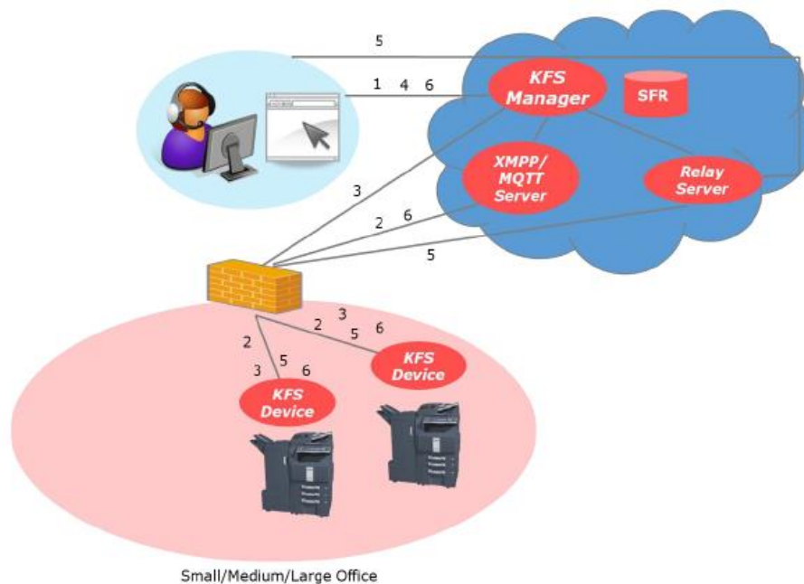
Figure 11 Communication flow of remote panel
