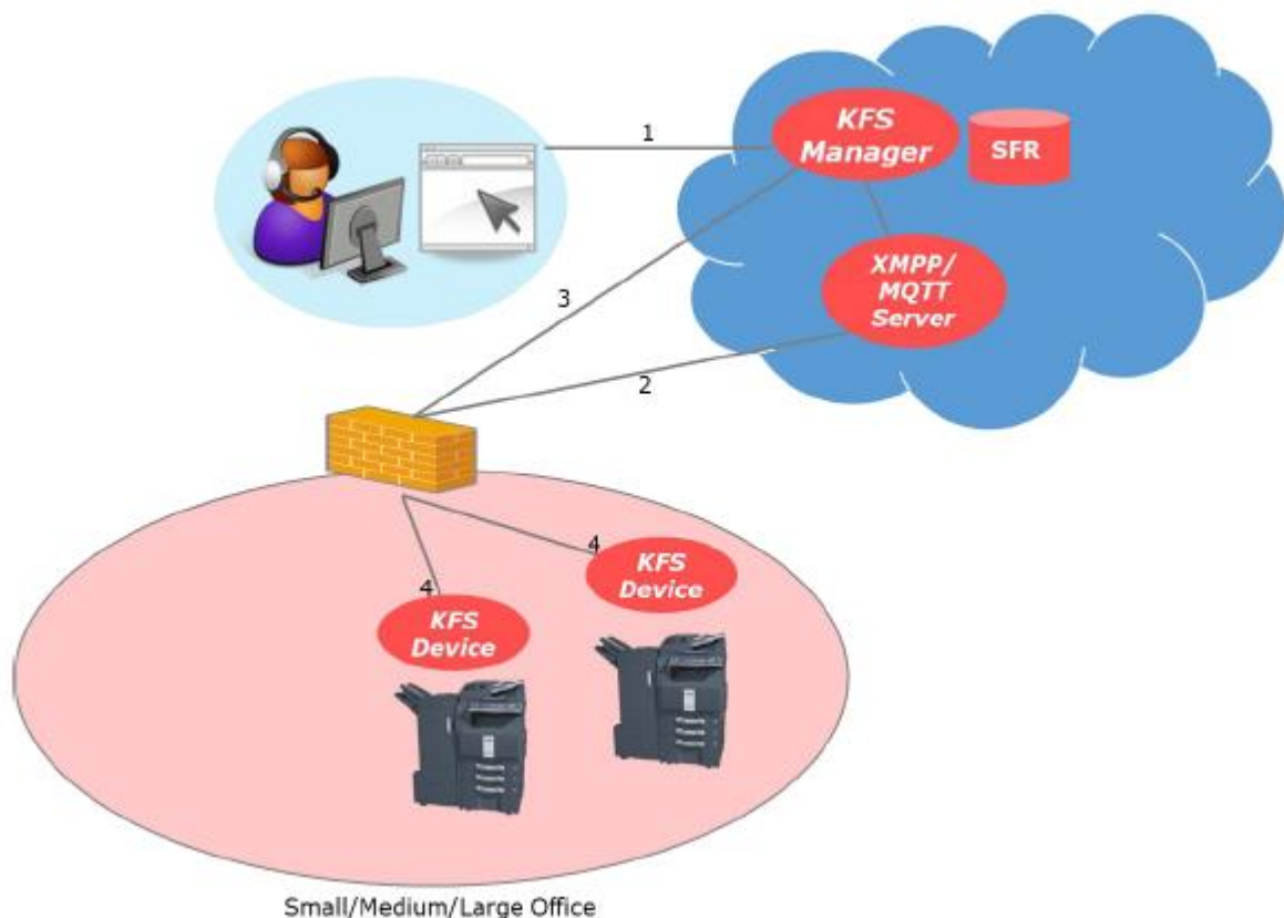
Figure 6 Communication flow of firmware upgrade from TA/UTAX Fleetmanager Gateway/ TA/UTAX Fleetmanager Device
